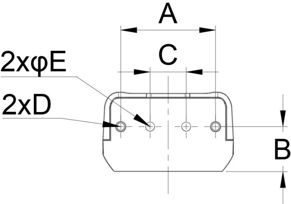
Figure 2-2 DM-Tac W connector mounting interface
